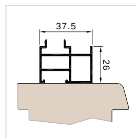
Adapterschiene ADS26Z
