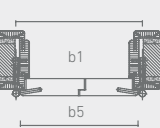
Horizontal section of the frame (RF) Double leaf, rebated
