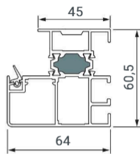
Aluminium-Zarge A2
