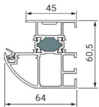
Aluminium-Zarge A1
