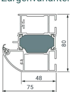
Aluminium-Zarge A3
