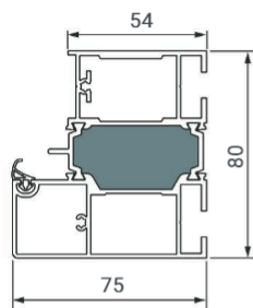
Aluminium-Zarge A4
